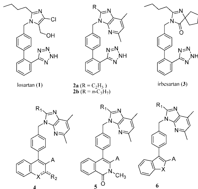
Chart 1. Structures of Compounds 1–6
