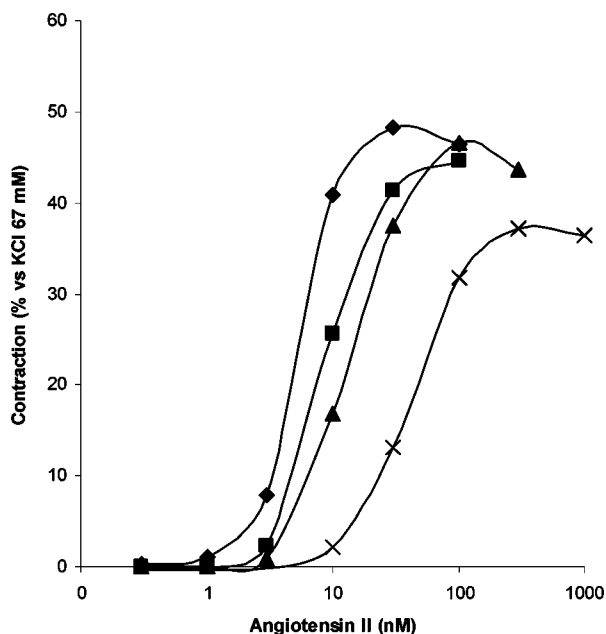
Figure 5. Concentration–contractile response curves for Ang II in isolated rabbit aortic strips, in the presence of different concentrations [10 nM (■), 30 nM (▲), or 100 nM (×)] of compound 8a or of its vehicle (◆).
