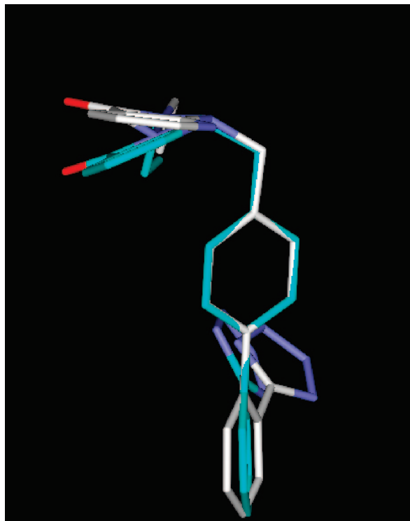
Figure 4. Superposition of 7a crystallographic structure (white) with a low energy conformer of 7q (cyan). This result suggests that 7q can populate the solid state conformation of 7a . Thus, the difference in the AT 1 receptor affinity between 7a and 7q is probably connected to the relative orientation of the pendent bicyclic system determined by the linker geometry (a sp^3 carbon in the case of 7q and a partially pyramidal nitrogen atom for 7a ).
