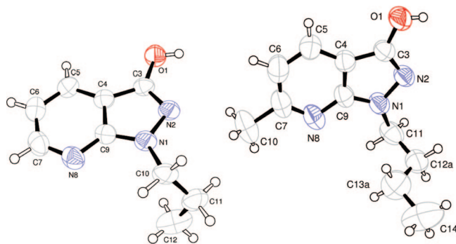
Figure 3. Crystal structure of pyrazolo[3,4- b ]pyridine derivatives 30 (left) and 32 (right). Ellipsoids enclose 50% probability.
