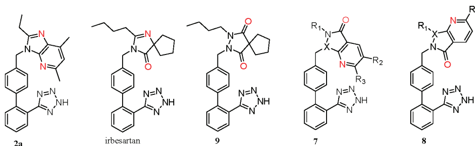
Chart 2. Structures of Compounds 2a , 7–9 , and Irbesartan a
