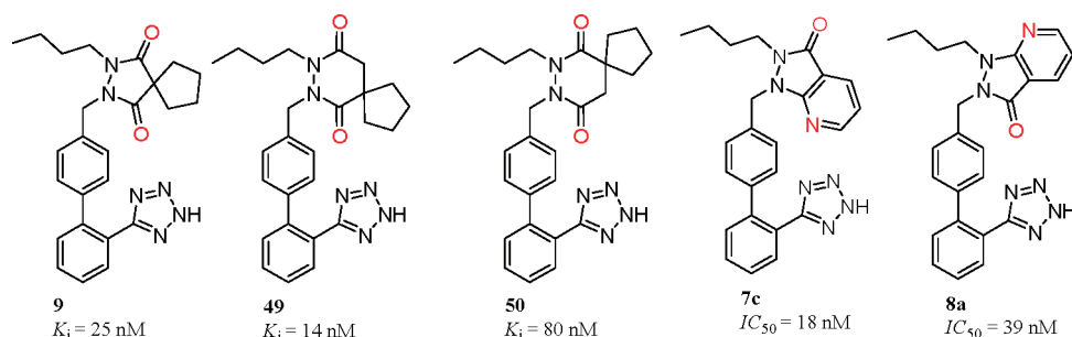
Chart 3. Structures of Compounds 7c , 8a , 9 , 49 , and 50 a
