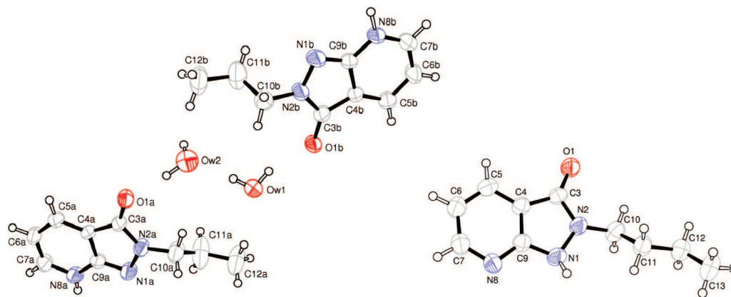
Figure 1. Crystal structure of pyrazolo[3,4- b ]pyridine derivatives 16a ·H 2 O (left) and 16c (right). Ellipsoids enclose 50% probability.
