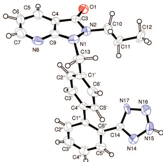
Figure 2. Crystal structure of target compound 7a . Ellipsoids enclose 50% probability.
